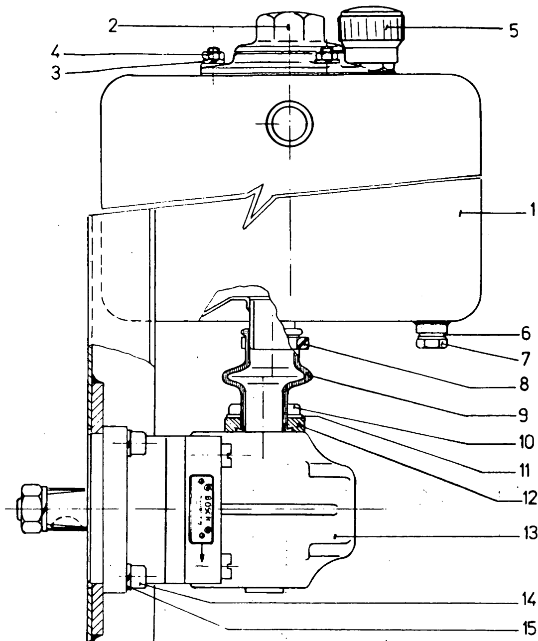
HYDR. POMP, RESERVOIR & FILTER 332651 - HYDR. PUMP, RESERVOIR & FILTER 332651 POMPE HYDR. RESERVOIR & FILTRE 332651 - HYDRAULIKPUMPE, ÖLBEHALTER & FILTER 332651
